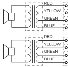
Fig. 2 - Circuit Diagram
