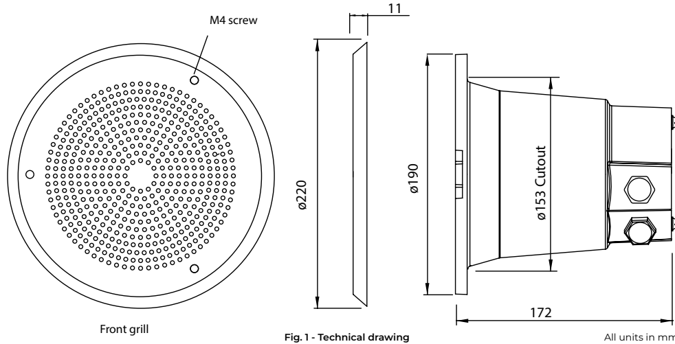
Fig. 1 - Technical drawing
