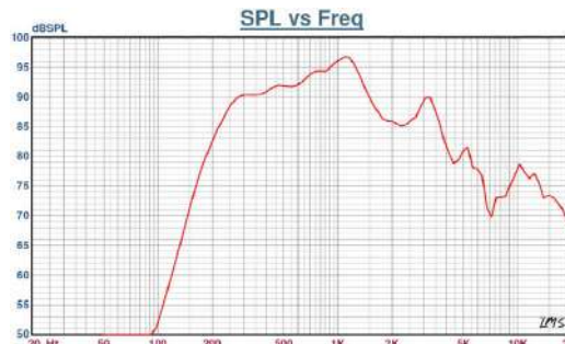
Fig. 3 - SPL at 1W/1m
