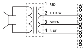
Fig. 2 - Circuit Diagram
