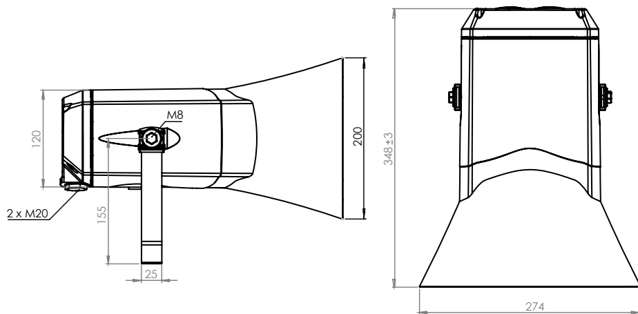
Fig. 1 - Technical drawing
