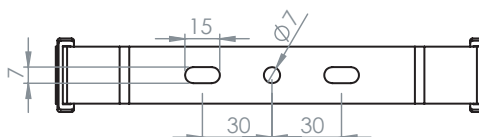
Fig. 5 - Hole placement - Stainless steel bracket
