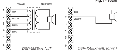
Fig. 2 - Circuit Diagram
