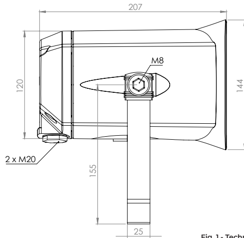
Fig. 1 - Technical drawing
