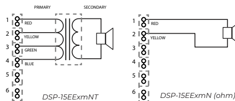
Fig. 2 - Circuit Diagram
